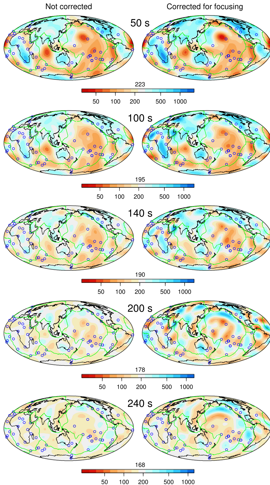
Figure C1. Maps of lateral variations of Q . Left column: maps are corrected for all effects except focusing (see eq. 1); right column: maps also include the focussing correction. Although the focussing corrections are visible on the maps, these corrections remain moderate. Hotspot locations are in blue (Müller et al. 1993), plates in green.
