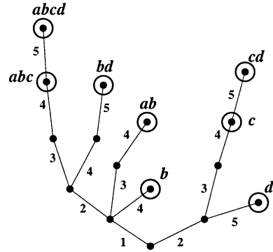
Fig. 2. The nodes with circle correspond to elements of \mathcal{F} , where the sequence a_1 a_2 \dots a_k are elements of \mathcal{B} with \bigcup_{i=1}^k a_i is the set of labels on the path to the root.
