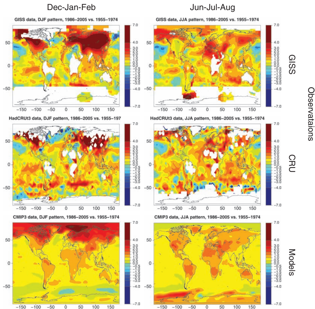
FIGURE 4.3 Relative patterns of warming (normalized to one for the globe), for December-January-February (left) and June-July-August (right) for 1955-2005 (obtained as differences between 20-year average temperatures for 1986-2005 and 1955-1974). The top two panels show results from two instrumental temperature records, NASA GISS and CRU. White indicates regions where data are not available. The bottom panels show results for the Climate Modelling Intercomparison Project (CMIP3) multi-model ensemble. Patterns expected from projections for the 21st century are largely similar to those shown here, as seen in Figure 4.1.
