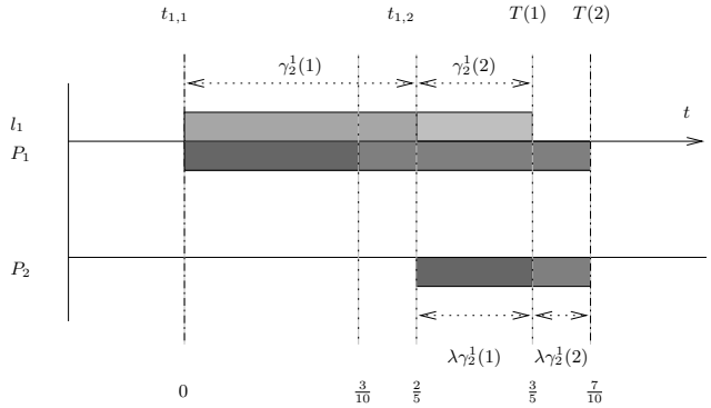
Figure 2. A possible schedule when \lambda = \frac{1}{2} .
