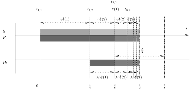
Figure 4. The schedule of [19] for \lambda = \frac{1}{2} .
