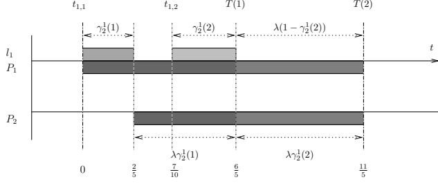
Figure 3. The schedule of [19] for \lambda = 2 .
