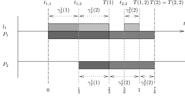
Figure 5. The schedule of [19] for \lambda = 1 .
