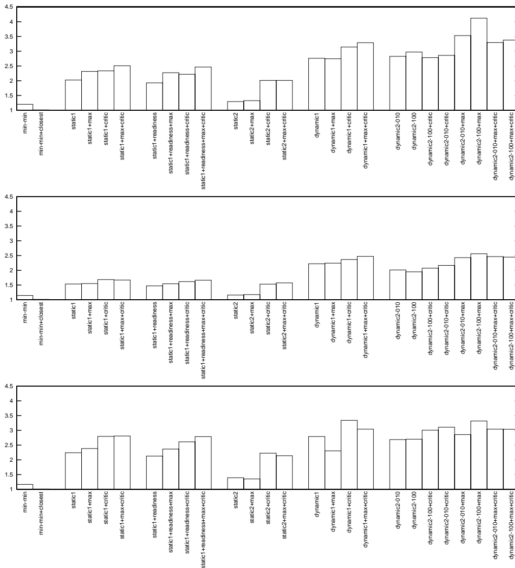
Figure 13: Relative performances of the schedules produced by the different heuristics ( except random ) average on the four types of graphs and three communication ratios, for the three types of platform graphs, from top to bottom: clique, random tree, and ring.
