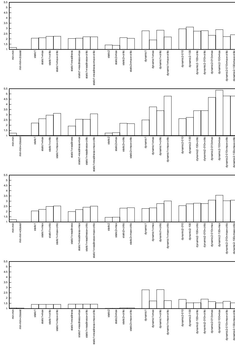
Figure 9: Relative performances of the schedules produced by the different heuristics ( except random ) average on three communication to computation ratios and three types of platform graphs, for the four types of graphs (from top to bottom: Two-one , Random , Partitioned , and Forks ).
