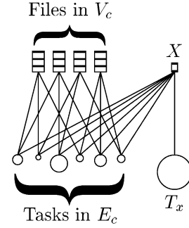
Fig. 4. The bipartite application graph used in the proof of Theorem 1, with |V_c| = 4 .
