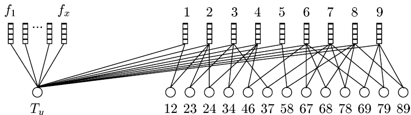
Fig. 5. The bipartite application graph used in the proof of Theorem 2.
