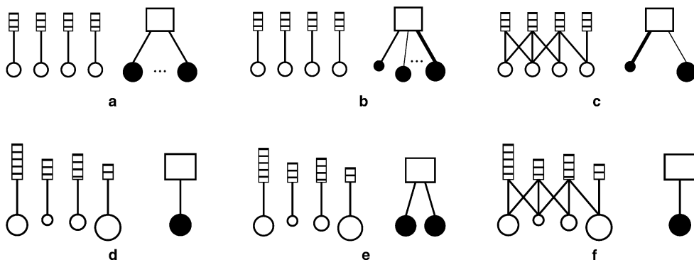
Fig. 3. Complexity results for the problem of scheduling tasks sharing files: (a) polynomial (round-robin); (b) polynomial [8]; (c) NP-complete (this paper); (d) polynomial [9] (e) NP-complete (2-PARTITION) (f) NP-complete (this paper).
