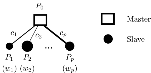
Fig. 2. Heterogeneous fork-graph.
