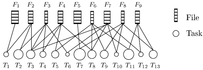
Fig. 1. Bipartite graph gathering relations between files and tasks.
