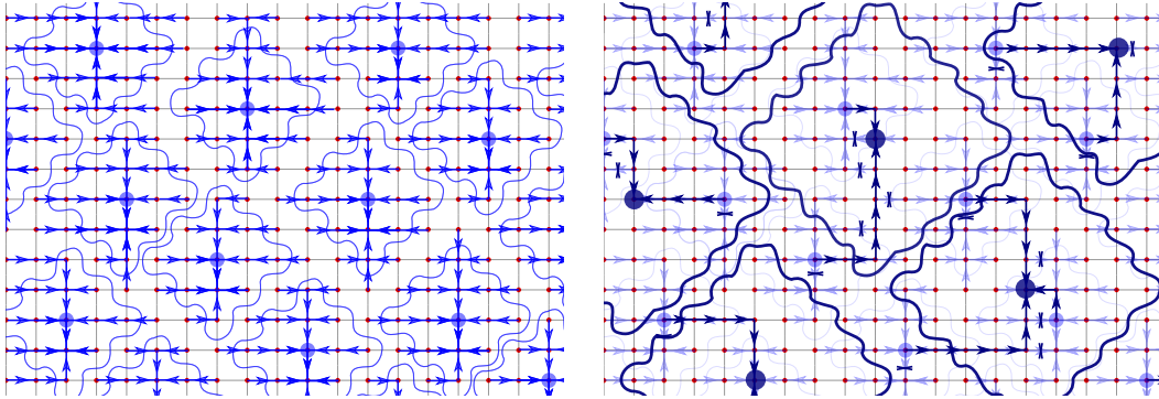
FIGURE 1. A_0 (red), A_1 (blue) and f_0 (blue arrows) – A_2 and f_1 (deep blue)
