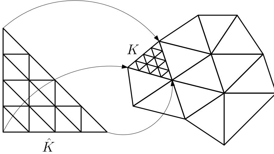
FIGURE 5.2. Left: the standard simplex \widehat{K} has been refined twice. Right: an unstructured coarse mesh, and the image of the twice-refined standard simplex through the affine mapping F_K for one particular coarse element K .
