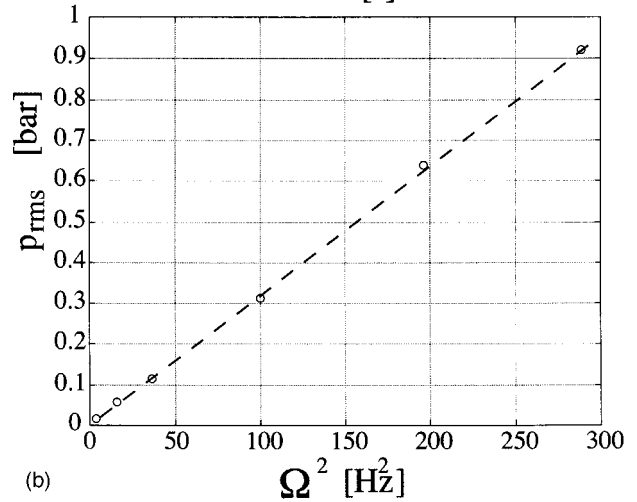
FIG. 5. (a) Time variation of the pressure measured at the flow wall ( \Omega=17 Hz); (b) evolution with the disks’ rotation rate of the rms amplitude of the pressure fluctuations. The dashed line corresponds to the quadratic law p_{rms}/\Omega^2 = 3.2 \times 10^{-3} [bar/Hz 2 ].
