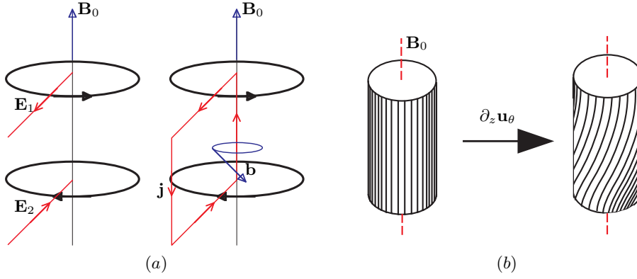
Fig. 3. Sketch of the omega effect produced by differential rotation, considered in (a) from the point of view of induction e.m.f. and induction currents, and in (b) from the point of view of magnetic field lines distortion by the velocity gradients.
