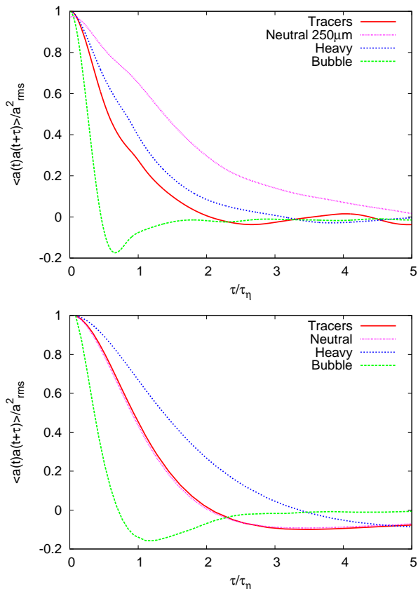
FIG. 3: Autocorrelation coefficients of the accelerations: (top) Data from experiments at Re_\lambda = 850 . (bottom) Data from DNS of homogeneous isotropic turbulence at Re_\lambda = 180 . For the (\beta, St) values we refer to table I.
