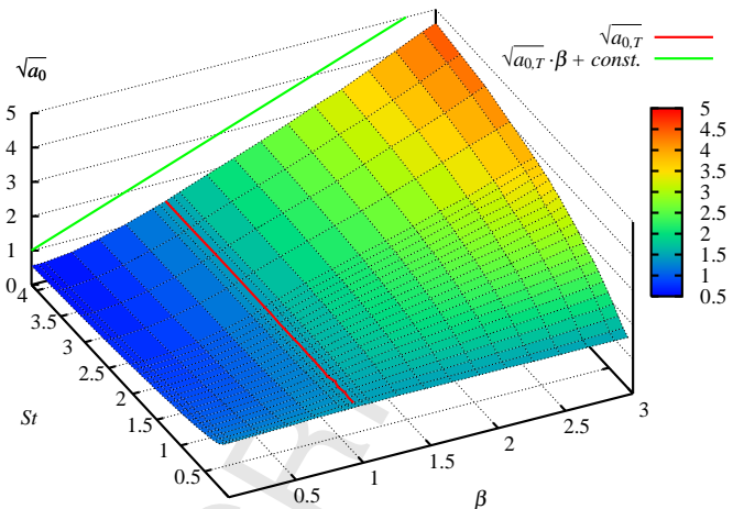
FIG. 4: Behavior of the normalized root mean square acceleration \sqrt{a_0} = (\langle a^2 \rangle \epsilon^{-3/2} \nu^{1/2})^{1/2} as a function of both St and \beta for a Re_\lambda = 75 DNS. Iso-contour for \sqrt{a_{0,T}} (red) and the line \sqrt{a_{0,T}} \cdot \beta + \text{const.} (green) are also reported. Note that a_0 does not depend on St for neutral ( \beta = 1 ) particles. While it is always reduced/enhanced for heavy/light particles. For large particles ( St \simeq 4.1 ) we find \sqrt{a_0} \simeq \beta \sqrt{a_{0,T}} .
