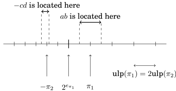
Fig. 1. Case \pi_1 = 2^{e_{\pi_1}} \cdot (1 + 2^{-p+1}) .
