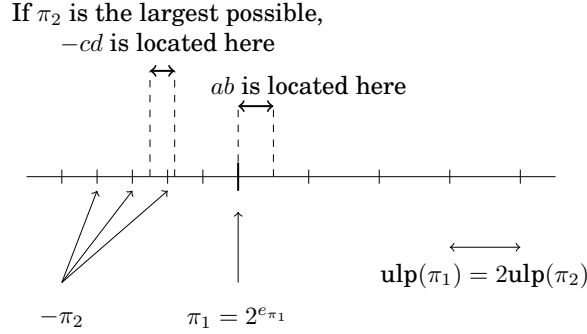
Fig. 2. Case \pi_1 = 2^e \pi_2 .
