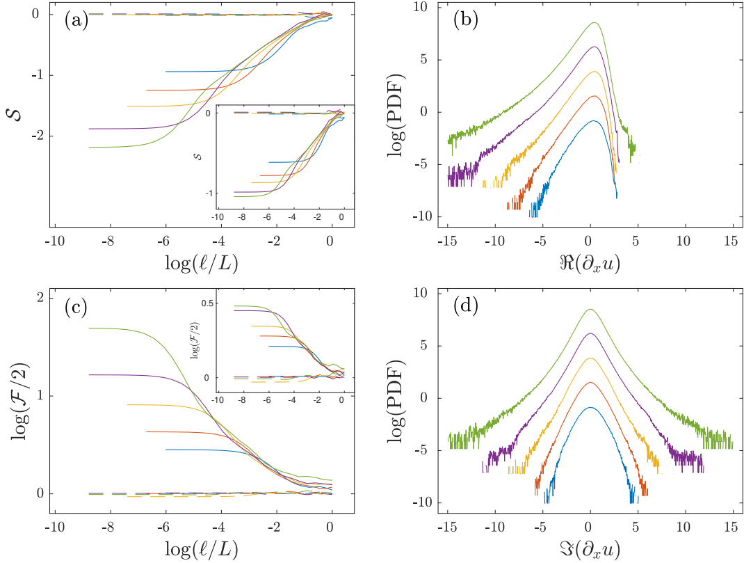
FIGURE 5.2. (a) and (c): similar plots as in Fig. 5.1(d), for the same values of the parameters, using the same colors and representing \gamma = 0 with dashed lines, and \gamma = \sqrt{0.02} with solid ones, but concerning the increment skewness \mathcal{S}(\ell) (Eq. 5.6) in (a), and flatness \mathcal{F}(\ell) (Eq. 5.7) in (c). Corresponding insets show the same statistical quantities but for a smaller value of the parameter \gamma = \sqrt{0.01} . (b) and (d): histograms of the values of the real \Re \partial_x u_{H,\gamma,\nu} and imaginary \Im \partial_x u_{H,\gamma,\nu} parts of the derivative of the solution, with the same parameters as former figures but for the single value \gamma = \sqrt{0.02} . For the sake of clarity, histograms correspond to unit-variance probability density functions, and are arbitrary vertically shifted (see text).
