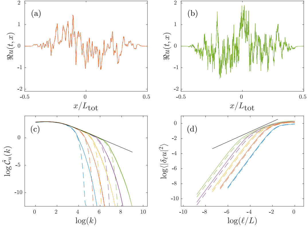
FIGURE 5.1. Local and statistical behaviors of the solution u_{H,\gamma,\nu}(t, x) detailed in Proposition 5.1. (a): spatial profiles of \Re u_{H,\gamma,\nu}(t, x) at a given time t in the statistically stationary regime for L = L_{\text{tot}}/10 , c = 10 , H = 1/3 , \nu = 10^{-6} , with \gamma = 0 (dashed line) and \gamma = \sqrt{0.02} (solid line). (b): same plot as in (a), but for a lower value of viscosity \nu = 10^{-9} . (c): estimations of the power spectrum based on the averaged periodograms (see text) of the solution for various values of viscosity \nu = 10^{-5} , 10^{-6} , 10^{-7} , 10^{-8} and 10^{-9} (from left to right), using dashed lines for \gamma = 0 , and a solid ones for \gamma = \sqrt{0.02} . We superimpose with a solid black line the asymptotic prediction made in Eq. 3.16, which has been obtained in the Gaussian and fractional case, properly weighted by a multiplicative factor to take the truncation of the force into account (see text). (d) Similar plot as for (c) but for the second order structure function, i.e. the variance of the increments, following an averaging procedure detailed in the text. We superimpose the expected asymptotic power-law behavior, given in Eq. 3.17, which is properly weighted (see text) and represented by a solid black line.
