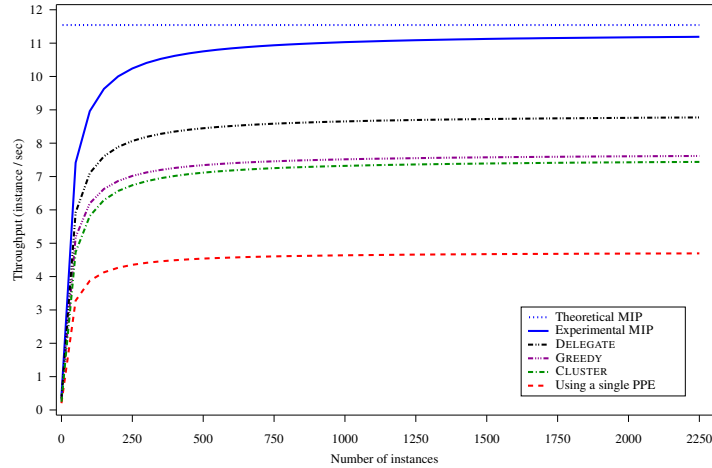
Figure 10: Throughput achieved depending on the length of the stream, using the task graph described in Figure 9(b), with a CCR of 0.004, on the QS 22 using all 16 SPEs.
