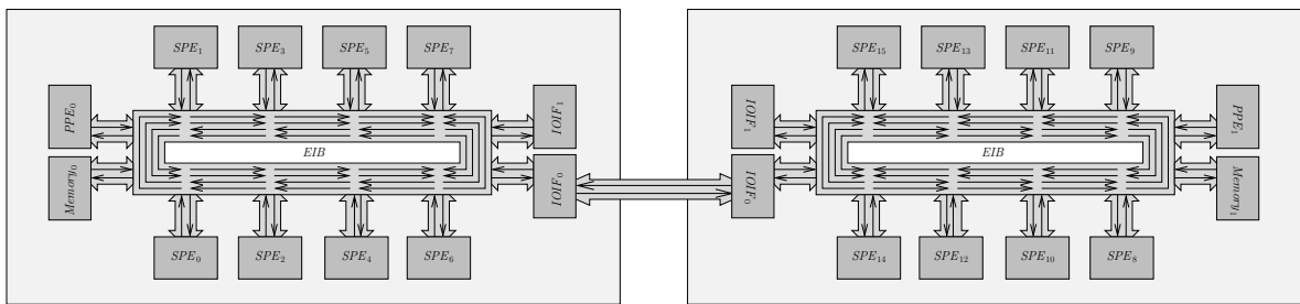
Figure 2: Schematic view of the QS 22.
