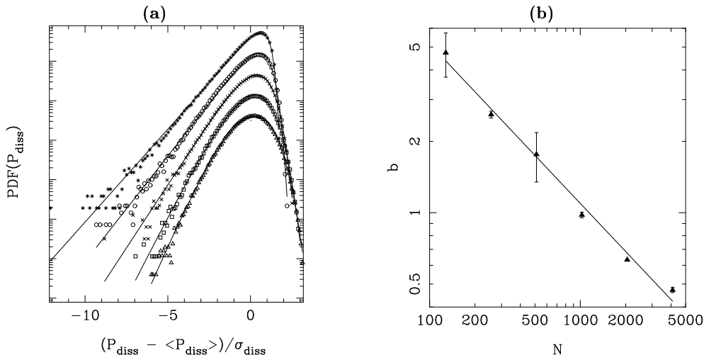
Fig. 3 – a) Probability distribution function (PDF) of the dissipated power P_{diss} for different system sizes: from top to bottom N = 256, 512, 1024, 2048, 4096 . The parameters of the model are \omega_0^2 = 1 , K = 1 , \nu = 5 \cdot 10^{-5} . The points correspond to histograms deduced from the numerical simulations and the full lines are fits with the generalized Gumbell distribution. For a better lisibility, each histogram is shifted by -0.5 unit along the vertical axis. b) Variation of the parameter b of the generalized Gumbell distribution versus the system size N in a log-log scale. The error bars correspond to extreme values obtained in different simulations.
