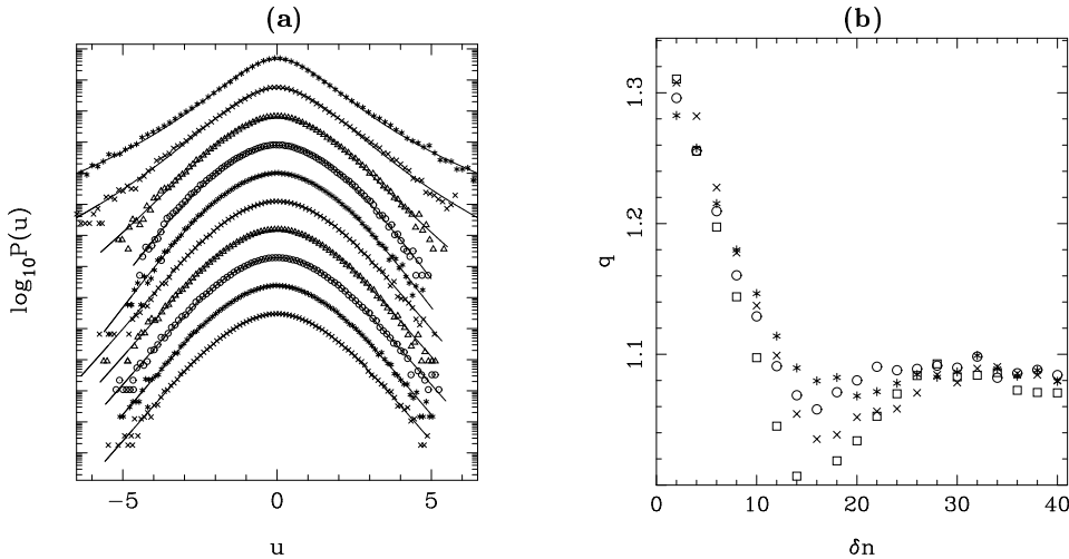
Fig. 2 – (a) Probability density functions of the velocity differences for \delta n = 2 (top plot) to \delta n = 40 (bottom plot), by steps of \delta n = 4 . The points correspond to the histograms obtained by numerical simulations and the full lines are the fits of \tilde{P}(\tilde{u}) according to Eq. (2). The parameters of the model are N = 256 , \omega_0^2 = 1 , K = 1 , \nu = 10^{-4} and A = 0.12 . The reference site is n_0 = 57 . For better lisibility, each distribution is shifter by -0.5 units. (b) Variations of the fitting parameter q versus \delta n/\nu for different viscosity parameters ( \nu = 5 \cdot 10^{-5} , circles \nu = 1 \cdot 10^{-4} , stars, \nu = 5 \cdot 10^{-4} , x, \nu = 2 \cdot 10^{-3} , squares)
