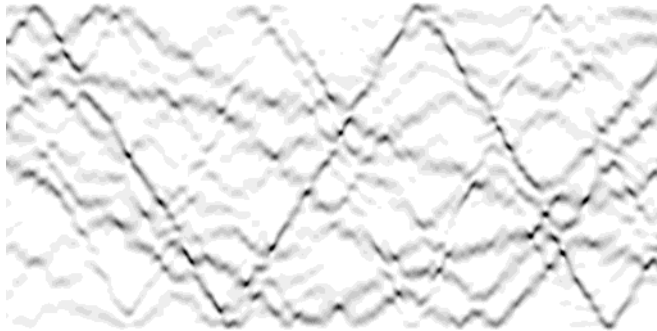
Fig. 1 – Energy density in a N = 256 -particle lattice excited by a single mode with p = 8 , A = 0.12 . The parameters of the model are \omega_0^2 = 1 , K = 1 , \nu = 5 \cdot 10^{-4} . The spatial dependence of the energy per unit celled e_n(t) is shown with a grey scale (white corresponding to 0 and black to a high energy density). The horizontal axis corresponds to time and extends over a time interval of 20 480 t.u., and the vertical axis gives the position n in the lattice.
