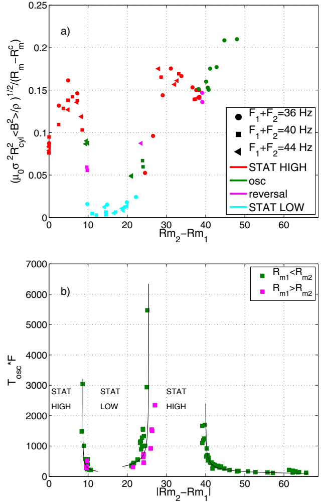
Fig. 6. (Color online) (a) Rescaling of the 3 transition plots of Figure 5, with \Delta R_m = R_{m2} - R_{m1} for the abscissa and |B|\sigma R_{cyl}\sqrt{\mu_0/\rho}/(R_m - R_m^c) for the ordinate ( R_m^c = 39 ). Symbols correspond to the different values of R_m , colors show the different dynamo regimes. (b) Evolution of the period of oscillations on either side of several windows of stationary dynamos. In this plot, since the oscillations period are not expected to depend on the sign of \Delta R_m all data points are shown, using different colors for points corresponding to \Delta R_m positive and negative. The solid lines are (|\Delta R_m| - |\Delta R_m^c|)^{-1/2} fits, where \Delta R_m^c is the value of \Delta R_m at the onset of each of the 3 transitions that display a period divergence.
