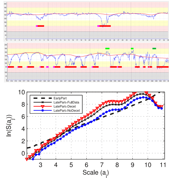
Figure 4: Long term time evolution of \hat{H} . Top: Two windows of 30-min (taking place 5 hours (top) and 40 minutes before delivery (bottom)) from 6-hour long recording (FIGO-TP7). Bottom: Wavelet spectra for early (black dotted line) and late (black solid line) window. Conditional wavelet spectra computed from the second block are also superimposed.
