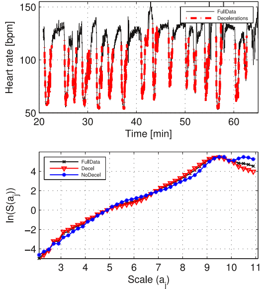
Figure 3: FHR time series (FIGO-FP14) with automatically detected decelerations (top) and comparison of the wavelet spectrum against the wavelet spectra ( S(a) ) conditioned to the presence ( S_d(a) ) and absence ( S_{nd}(a) ) of decelerations.
