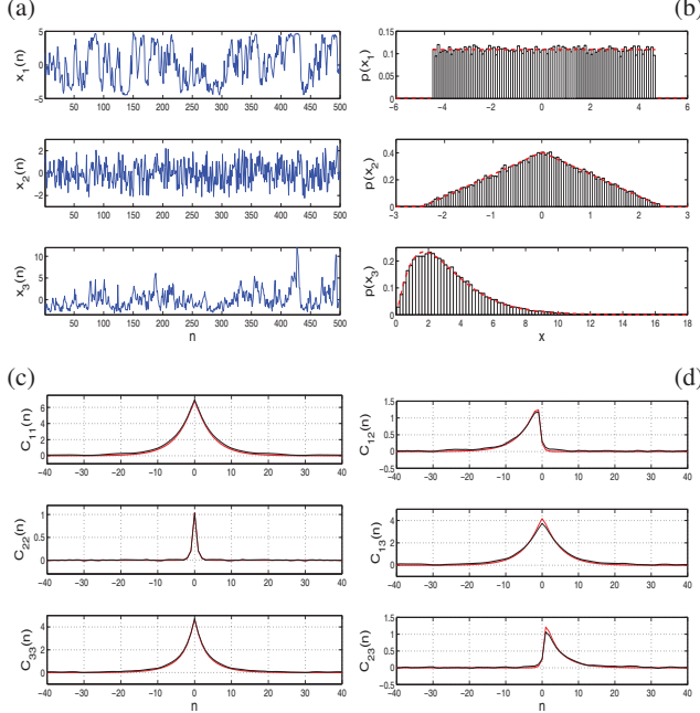
Fig. 1. Example with ALGORITHM 1: Covariance of a Moving Average and marginals as defined in Section 2.3. (a) Zoom on the time series. (b) Empirical estimations (bars) and prescribed forms (dashed red lines) for the marginal distributions. (c) Auto-covariances and (d) Cross-covariance for surrogates (black) and model (red). All empirical estimates on surrogates are done with N = 2^{15} .
