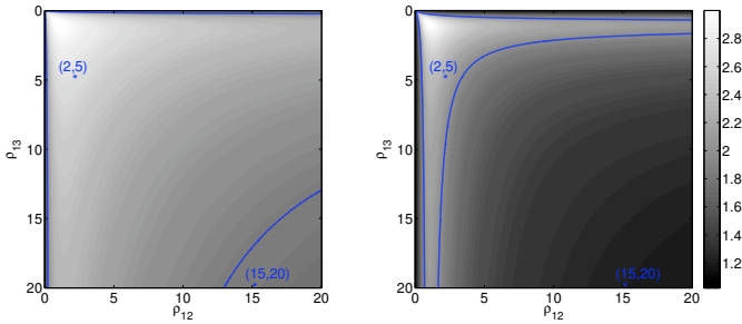
Fig. 1. Estimated number of components N(t) in the case K(t) = 3 , as a function of the amplitude ratios \rho_{12}(t) and \rho_{13}(t) , for a Rényi entropy of order \alpha = \frac{1}{2} (left) and \alpha = 2 (right). The isocontours N(t) = 2 are superimposed as full blue lines. The two specific cases that will be considered in Section 4 are reported as blue dots.
