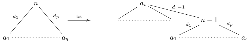
Fig. 1. Rewriting rule on skeletons
