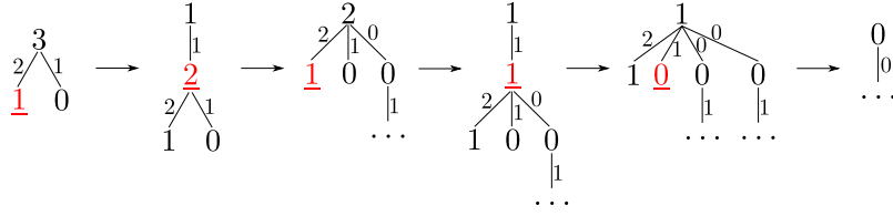
Fig. 2. Example reduction sequence on bounding skeletons
