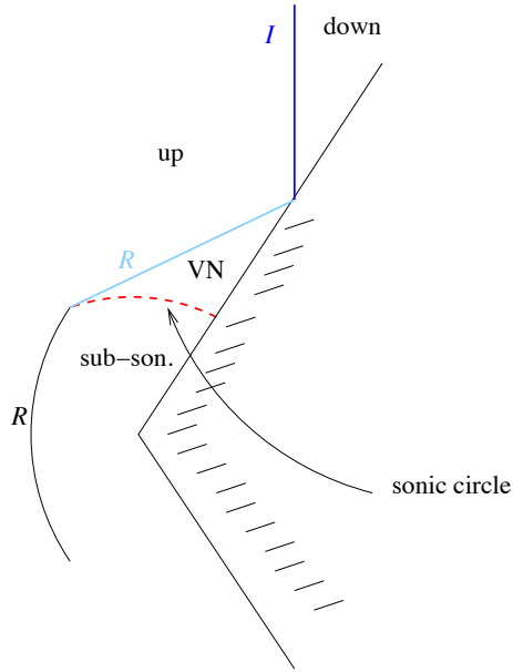
Figure 1: The Regular Reflection. The solid wedge is at right. The reflected shock R is straight until it meets S . Then it becomes a curve.
