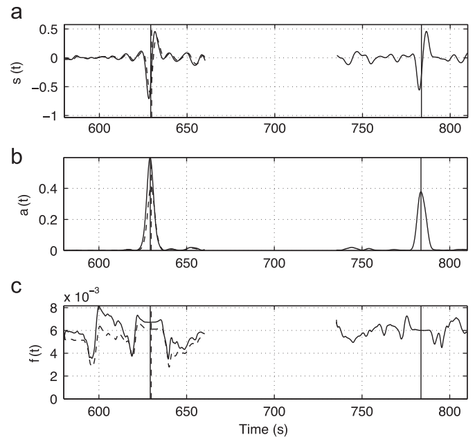
Fig. 1. Instantaneous frequency matching (IFM) method. First, we pick the S and ScS seismic phases by taking the maximum of the envelope (middle panel). Then we compute the instantaneous frequency and compare its value in the time domain at the arrival times of the two seismic waves. The S wave is attenuated using the causal operator D(\omega) , Eq. (2), in the frequency domain for a range of \delta t_{\text{ScS-S}}^* until the instantaneous frequencies are matched in the time domain. The dashed lines correspond to the attenuated seismogram, amplitude and instantaneous frequency. The \delta t_{\text{ScS-S}}^* in this example is 0.6 s. (a) Filtered [0.018 0.2] Hz and anisotropy corrected seismograms, (b) envelope and (c) instantaneous frequency (Hz).
