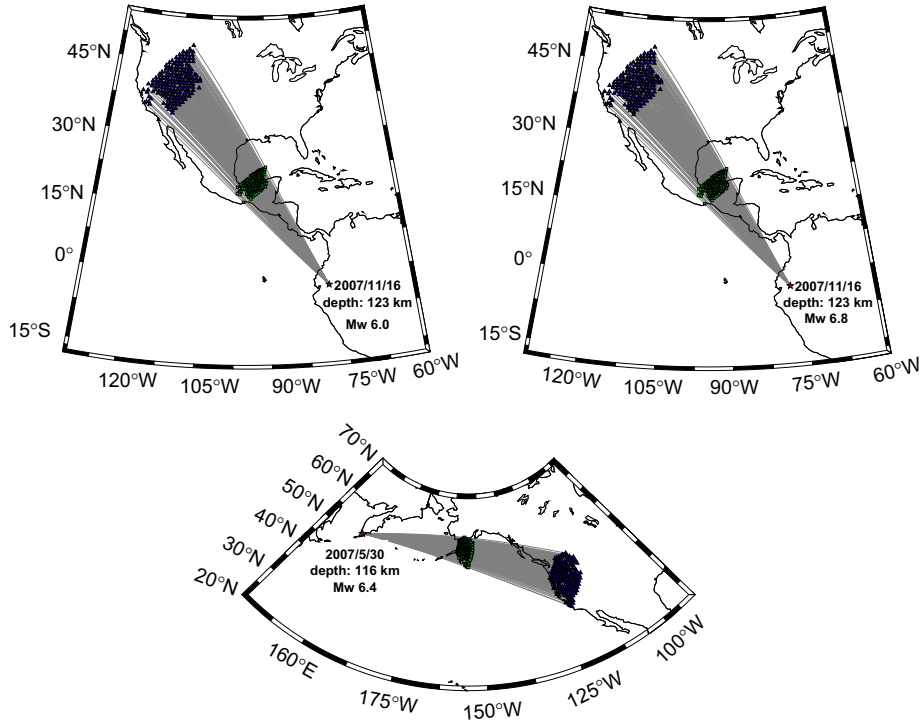
Fig. 4. Selected high quality data recorded by the USArray. (top) Core reflection points under Central America. (bottom) Core reflection points under Alaska. Blue triangles are the stations, red stars the epicenters, green squares the ScS core reflection points and grey lines the seismic paths projected at the surface. (For interpretation of the references to color in this figure caption, the reader is referred to the web version of this article.)
