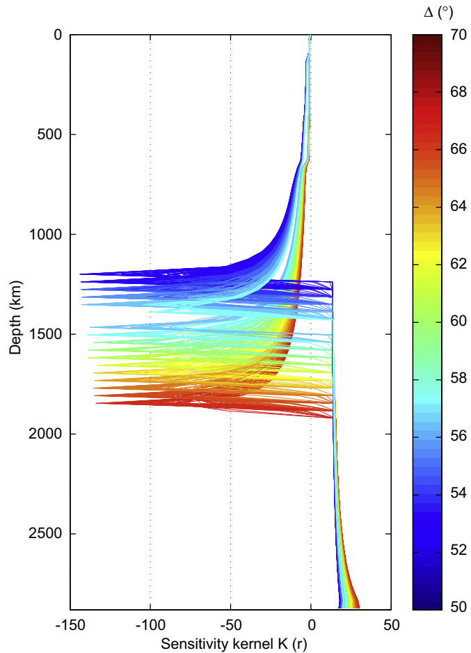
Fig. 7. Anelastic delay time sensitivity kernels. The colorbar indicates the epicentral distance. The sensibility is maximum and negative at the location of the turning points of the S wave while the sensibility is positive and somewhat reduced at the base of the mantle. It also shows that differential anelastic delay times are not sensitive to the attenuation structure of the lithosphere. (For interpretation of the references to color in this figure caption, the reader is referred to the web version of this article.)
