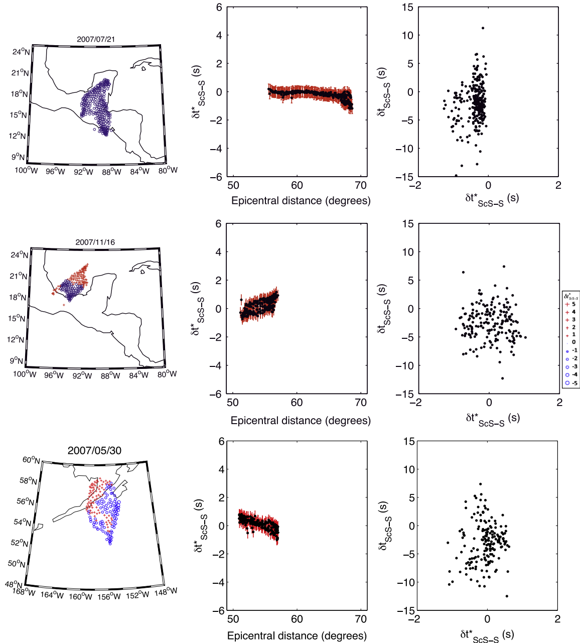
Fig. 6. Stacked anelastic delay times. (left column) Measurements plotted at the reflection point of the ScS on the CMB. (middle column) Measured \delta t_{ScS-S}^* versus epicentral distance. (right column) Elastic delay-times \delta t_{ScS-S} versus anelastic delay-times \delta t_{ScS-S}^* . Both quantities have been corrected using PREM and SAW24B16 for the propagation. The stacking highlights the revealed trends of the \delta t_{ScS-S}^* with the epicentral distance. No clear correlation is found between elastic and anelastic delay times.
