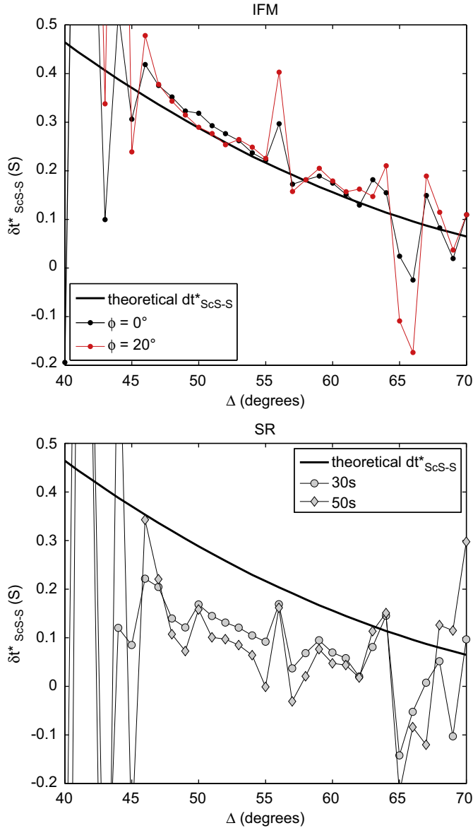
Fig. 3. Comparison of the SR and IFM methods. (top) Differential anelastic delay times \delta t_{ScS-S}^* obtained by the IFM method applied on the synthetic seismograms plotted in Fig. 2 for path azimuths \phi of 0^\circ (black dots) and 20^\circ (red dots). (bottom) Differential anelastic delay times \delta t_{ScS-S}^* obtained by the SR method applied on the set of synthetic seismograms with \phi = 0^\circ for two time windows, 30 s (circles) and 50 s (diamonds). The comparison of the results highlights the better accuracy of the measurements obtained with the IFM method. The two plots also illustrate the effect of interfering phases and of radiation pattern on the measurements. The presence of interfering phases around 45^\circ and 65^\circ significantly degrades the measurements, while the effect of the azimuth is negligible except when phases are interfering. The theoretical values of \delta t_{ScS-S}^* obtained using PREM parameters and Eq. (2) are plotted as black curve. (For interpretation of the references to color in this figure caption, the reader is referred to the web version of this article.)
