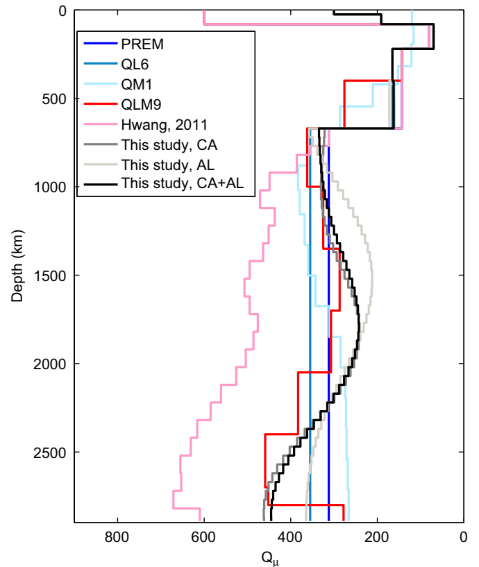
Fig. 8. Various radial Q_{\mu} models in the mantle. Our models (grey and black lines, CA for Central America and AL for Alaska) bear some similarities with the other body wave based models (red and blue curves) with a less attenuating bottom part of the lower mantle where the normal mode based models are more uniform. (For interpretation of the references to color in this figure caption, the reader is referred to the web version of this article.)
