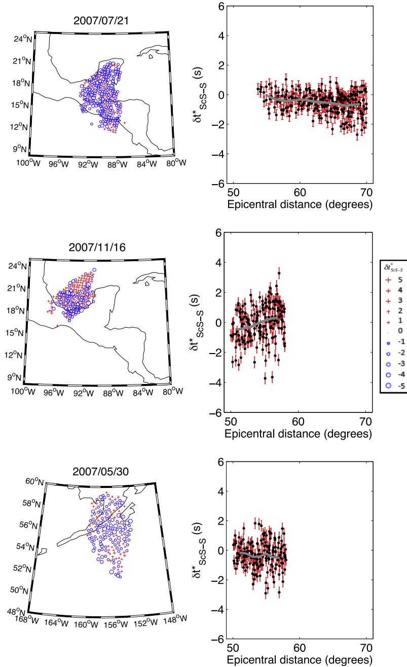
Fig. 5. Individual anelastic delay times. Measurements at the reflection point of the ScS on the CMB under Central America (top and middle) and under Alaska (bottom) for the three events considered in this study (see Fig. 4). The delays are corrected using PREM attenuation and the velocity model SAW24B16 (Mégnin and Romanowicz, 2000). (left column) Maps of the measured \delta t_{\text{ScS-S}}^* plotted at the reflection point of the ScS on the CMB. (right column) \delta t_{\text{ScS-S}}^* versus epicentral distances. The thick grey line represents the mean value. (For interpretation of the references to color in this figure caption, the reader is referred to the web version of this article.)
