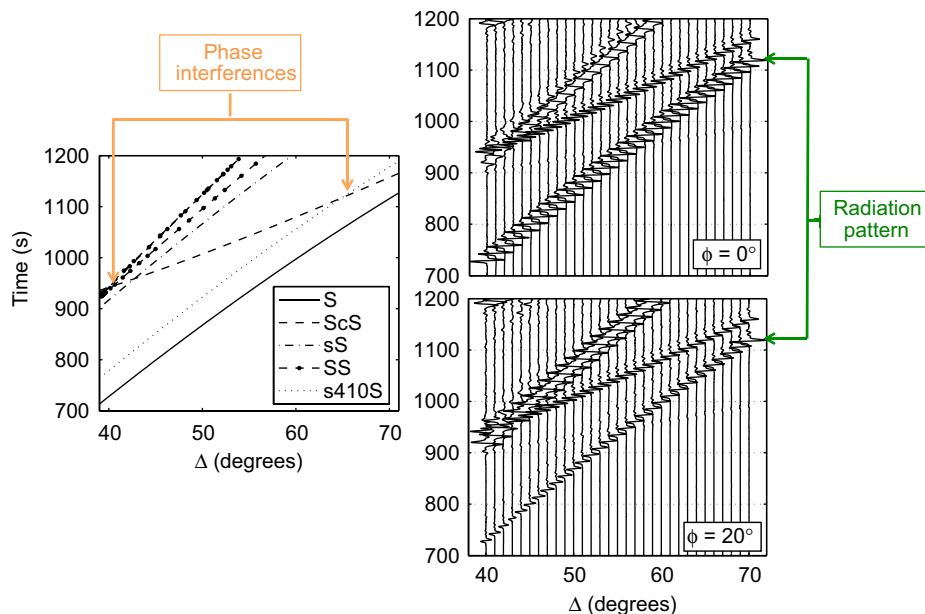
Fig. 2. Hodochrons of the synthetic seismograms. Two simulations for an event depth of 600 km, strike= 0^\circ , dip= 30^\circ and rake= 90^\circ and two path azimuths \phi = \{0, 20\}^\circ are shown. (left) Phases are interfering around 45^\circ (ScS, sS, SS) and around 65^\circ (ScS, s410S). (right) The change in path azimuth causes a significant decrease of the S amplitudes.
