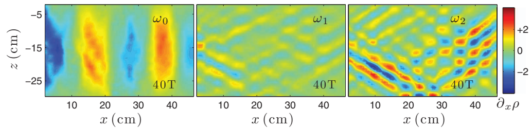
FIG. 2. Real part of the Hilbert transform of \tilde{\rho}_x at t = 40T (see Fig. 1 (right)) presented after filtering at \omega_0 = 0.95N (left), \omega_1 = 0.38N (center), and \omega_2 = 0.57N (right). Note that the shade scale (color scale) is the same as in Fig. 1.
