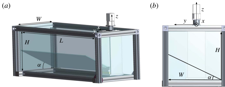
FIGURE 13. (Colour online) The canal-like geometry: perspective (a) and side (b) views of the experimental set-up. The slope and the wave generator are visible. The parameters used for the experiment are H = 360 mm, L = 1000 mm, W = 410 mm and \alpha = 23^\circ .
