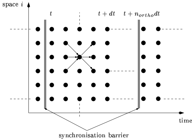
Figure 3: Reduced tasks graph of our program: both sub-graphs (system and tangent space) have been superposed. Reduced dependences are then (1, 1)^t , (1, 0)^t et (1, -1)^t . To avoid the use of an additional temporary array, the four phases of the perturbations evaluation for time t + dt that depends on the value of the system at time t are considered as atomic.
