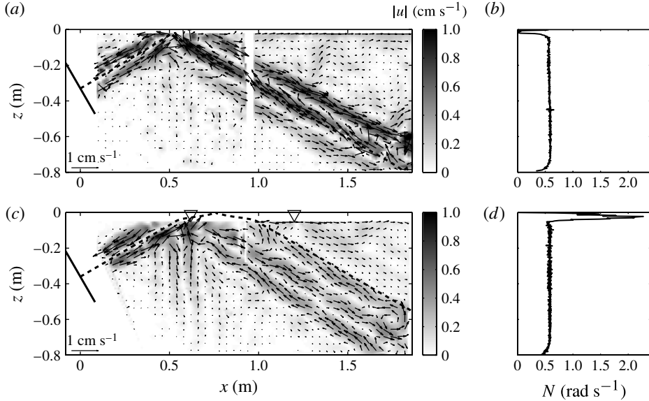
FIGURE 2. Comparison between experiments without ( a,b , EXP03) and with a pycnocline ( c,d , EXP08). The stratification profiles are shown in ( b ) and ( d ), and the corresponding measured velocity vectors and magnitude at t = 240 s after the start-up of the forcing in ( a ) and ( c ), respectively. The dashed lines represent the theoretical direction of internal-wave energy propagation, starting from the centre of the wavemaker, which is indicated by the solid line on the left. Insufficient overlap between the two cameras, around x = 0.9 m, leads to a gap in the velocity field in ( a ). The two inverted triangles in ( c ) indicate the positions of the ultrasonic probes at x = 0.62 m and x = 1.20 m.
