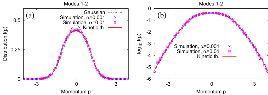
Figure 3. Stationary momentum distribution f(p) , on (a) linear, and (b) semi-log scales, for \alpha = 0.001 and 0.01 at kinetic temperature T = 0.75 . The plots correspond to modes 1 and 2 excited with amplitudes satisfying c_1 = c_2 = C(0)/4 , where C(0) = 2T . The data denoted by crosses and squares are results of N -body simulations of the stochastically forced HMF model with N = 10\,000 , \Delta t = 0.01 and 1000 independent realizations of the dynamics, while the red continuous lines refer to the theoretical prediction from the kinetic theory. For comparison, the black broken line shows the Gaussian distribution with the same kinetic energy (stationary state of the stochastically forced HMF model at T = 0.75 , c_0 = c_1 = 0 , c_2 = 0.75 , c_{k \geq 3} = 0 ).
