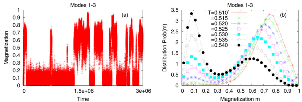
Figure 7. (a) Numerical simulation results for magnetization in the stochastically forced HMF model as a function of time at kinetic temperature T = 0.53 , with N = 5000, \alpha = 0.005, \Delta t = 0.01 , and with modes 1–3 excited, whose amplitudes satisfy c_1 = c_2 = c_3 = C(0)/6 , where C(0) = 2T . The figure shows clear signatures of bistability in which the system during the course of evolution switches back and forth between spatially homogeneous ( m \sim O(0) ) and inhomogeneous ( m \sim O(1) ) states. (b) Distribution \text{Prob}(m) of the magnetization m as a function of T at a fixed value of \alpha = 0.01 . The data are obtained from numerical simulation results similar to (a) for magnetization in the stochastically forced HMF model, with N = 5000, \Delta t = 0.01 , and with modes 1–3 excited, whose amplitudes satisfy c_1 = c_2 = c_3 = C(0)/6 , where C(0) = 2T .
