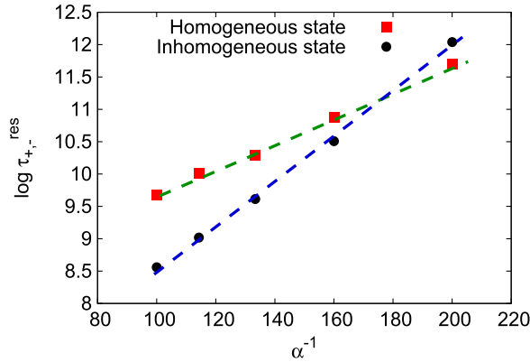
Figure 9. The plot shows as a function of 1/\alpha the log of the mean residence time \tau_{+,-}^{\text{res}} in the two bistable states, namely, the inhomogeneous ( m > 0 ) state and the homogeneous state ( m \approx 0 ). The plot is based on data obtained from simulations with modes 1–3 excited, whose amplitudes satisfy c_1 = c_2 = c_3 = C(0)/6 , where C(0) = 2T . Here, the kinetic temperature T = 0.53 , while \Delta t = 10^{-2} , N = 5000 . The straight line fits imply that \tau_{+,-}^{\text{res}} \sim \exp(1/\alpha) , in accordance with equations (41) and (42). That the slopes of the two straight lines in the plot are different could be due to the fact that the height of the barrier is different when observed from the inhomogeneous and the homogeneous state.
