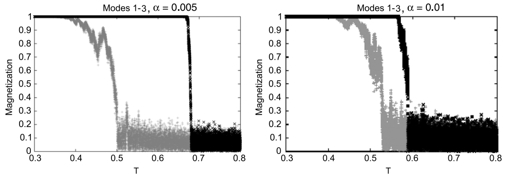
Figure 6. Numerical simulation results for magnetization in the stochastically forced HMF model as a function of adiabatically tuned kinetic temperature T for two different values of \alpha . In each case, the modes 1–3 are excited with amplitudes satisfying c_1 = c_2 = c_3 = C(0)/6 , where C(0) = 2T . In all cases, N = 5000, \Delta t = 0.01 , while the tuning rate for T is 10^{-5} . The gray points correspond to the case when the temperature is decreased from high values, while the black points correspond to the case when the temperature is increased from low values.
