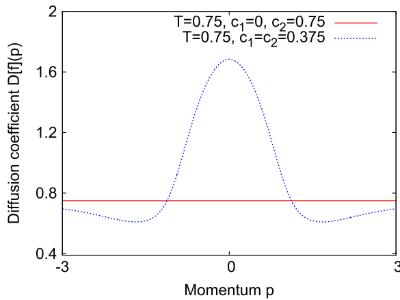
Figure 4. Diffusion coefficient D[f](p) for the stationary momentum distribution f(p) at kinetic temperature T = 0.75 , with c_0 = c_{k \geq 3} = 0 , and either (i) c_1 = c_2 = 0.375 , or (ii) c_1 = 0 , c_2 = 0.75 .
