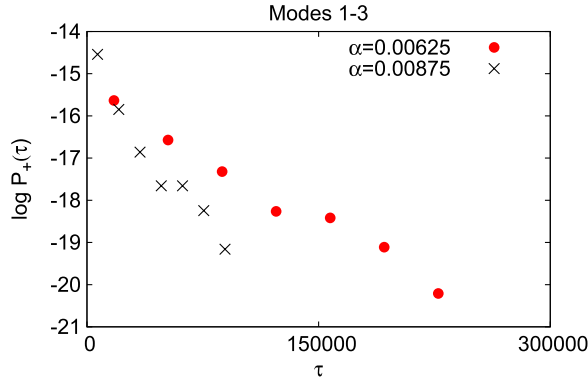
Figure 8. Distribution of the residence time \tau in the inhomogeneous state, for two values of \alpha . The data are obtained from simulations with modes 1–3 excited, whose amplitudes satisfy c_1 = c_2 = c_3 = C(0)/6 , where C(0) = 2T . Here, the kinetic temperature T = 0.53 , while \Delta t = 10^{-2} , N = 5000 .
