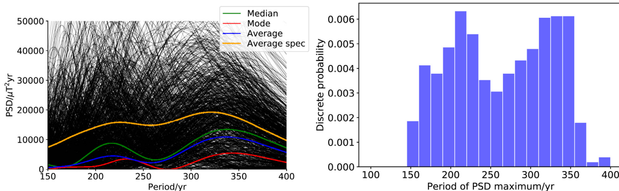
Figure 14. Power spectral density as a function of period for the AH-RJMCMC method applied to the Hawaii data set, restricted to the period 500–2000 AD. Left-hand panel: the PSD for each of the 1000 representative ensemble members are shown by thin black lines; the PSD for the median, mode and average are shown as green, red and blue respectively, while orange shows the average of the 1000 individual PSD curves. Right-hand panel: a normalized histogram of the period corresponding to the maximum PSD.
