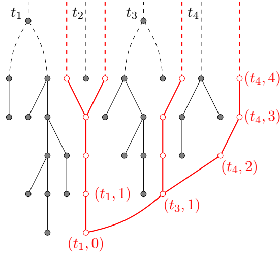
Figure 5: An infinite 1-admissible forest \mathbf{f} in which 4 trees t_1, t_2, t_3 and t_4 reach reverse height 4. In red, the tree \mathbf{U}(\mathbf{f}) and the names of some of its vertices. In the proof of Proposition 2.13 for r = 4 , the p_j^r are equal to 2, 1, 2 and 1 and the h(f_j) are equal to 4, 0, 3 and 2.
