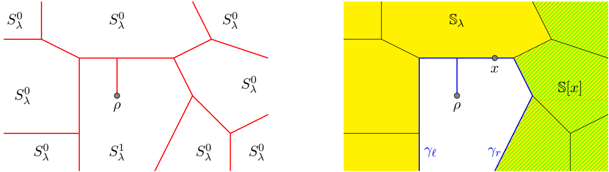
Figure 1: The strip decomposition of \mathbb{T}_\lambda . On the left, the tree \mathbf{T}_\lambda^g is in red. On the right \mathbb{S}_\lambda = \mathbb{S}[\rho] is colored in yellow. The part \mathbb{S}[x] of \mathbb{S}_\lambda that is shaded in green has the same distribution as \mathbb{S}_\lambda .
