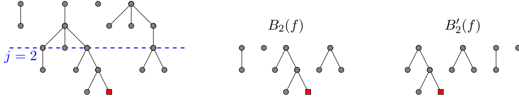
Figure 4: A forest f of height 4 and the forests B_2(f) and B'_2(f) . The ancestors lie on the top and the distinguished vertex is in red.
