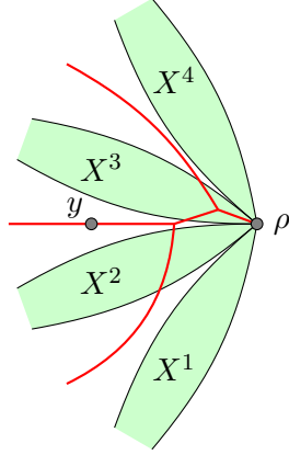
Figure 11: Sketch of the proof that \nu_\partial is nonatomic: if X^1, \dots, X^4 are four independent simple random walks, then there are three infinite leftmost geodesics (in red) between X^1 and X^4 , so there is a slice \mathbb{S}[y] there. The hulls of the four random walks are in green.
