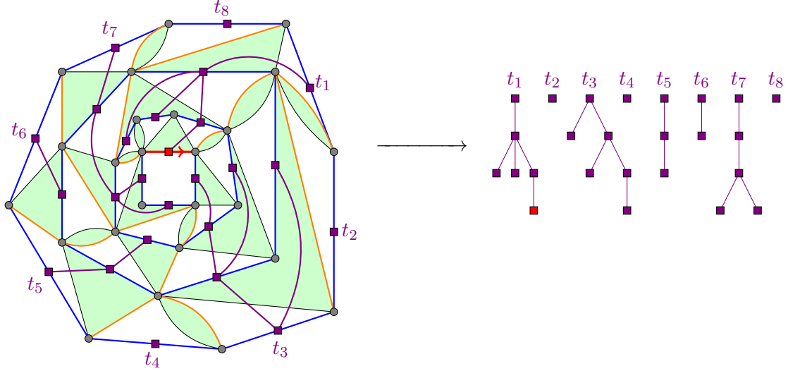
Figure 3: A triangulation of the cylinder \Delta and its skeleton \text{Skel}(\Delta) \in \mathcal{F}'_{4,8,3} in purple. The cycles \partial_j \Delta are in blue, and the root edge is in red. The leftmost geodesics from the vertices of \partial_* \Delta to \partial \Delta are in orange. The green holes must be filled by triangulations of polygons.
