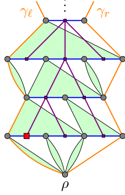
Figure 6: An infinite strip S and its skeleton.
