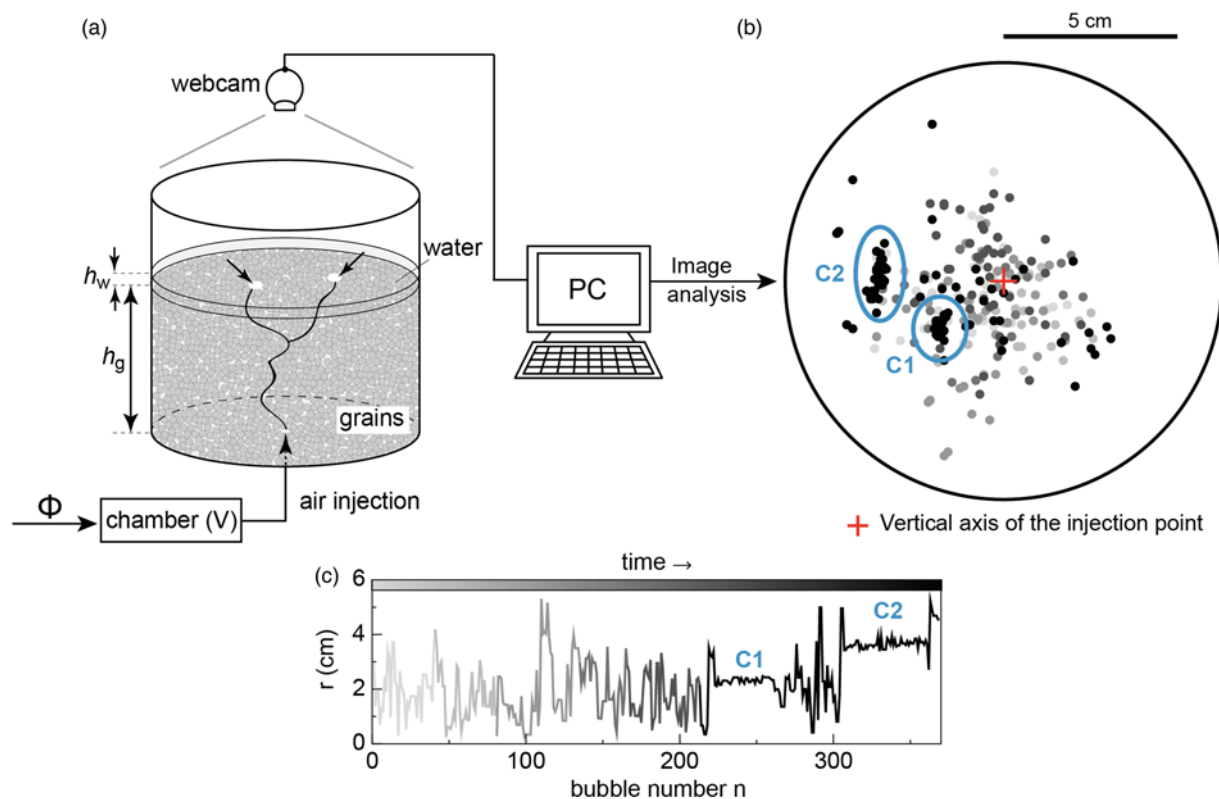
Fig. 10. Three-dimensional sandbox experiment (Varas et al. 2015). (a) Experimental setup. Air is injected at a constant flow rate \Phi at the bottom of an immersed granular column ( h_g is the height of grains and h_w the height of water above the granular bed). Bubble emission at the free surface is recorded by a webcam positioned over the experimental cell. (b) Detection of bubble emission at the free surface ( d = 318 \pm 44 \mu\text{m} , h_g = 14 \text{ cm} , h_w = 2 \text{ cm} , \Phi = 4.3 \text{ ml s}^{-1} ; the colour of dots from light grey to black is proportional to time). The system releases bubbles in different (uncorrelated) positions. For two significant periods of time, however, several successive bubbles are emitted in a narrow region (clusters C1 and C2). This indicates the formation of a gas channel fixed at depth (region C1), which then collapses before it can reopen in another region (C2). (c) Distance r between the bubble emission location and the centre of the cell (red cross in (b)) as a function of the bubble number n for the sequence presented in (b).
