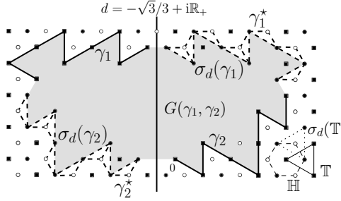
Figure 9: The graph G(\gamma_1, \gamma_2) with the two solid arcs \gamma_1 and \gamma_2 and the dashed arcs \sigma_d(\gamma_1) and \sigma_d(\gamma_2) . The dual arcs \gamma_1^* and \gamma_2^* are dotted.
