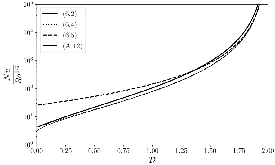
FIGURE 1. Prefactor of Ra^{1/2} in the Nusselt bound, in the limit of large values of (2 - \mathcal{D})Nu for a perfect gas with \gamma = 5/3 , computed from (6.4). The simpler expression computed from (6.5) is also shown as a function of \mathcal{D} . The thin line shows the bound (A 12) when s_0 is optimized (see appendix A).
