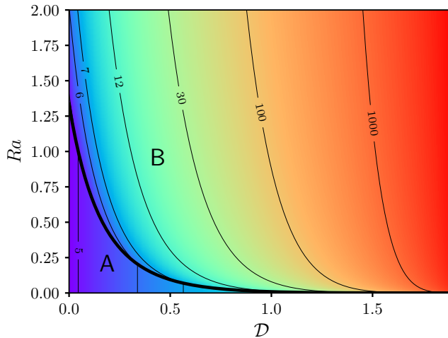
FIGURE 2. Isovalues of the bound of the Nusselt number (indicated by color level and a few isolines), for small Nusselt numbers (4.29) in zone A and large Nusselt numbers (6.2) in zone B, separated by the boundary (7.1).
