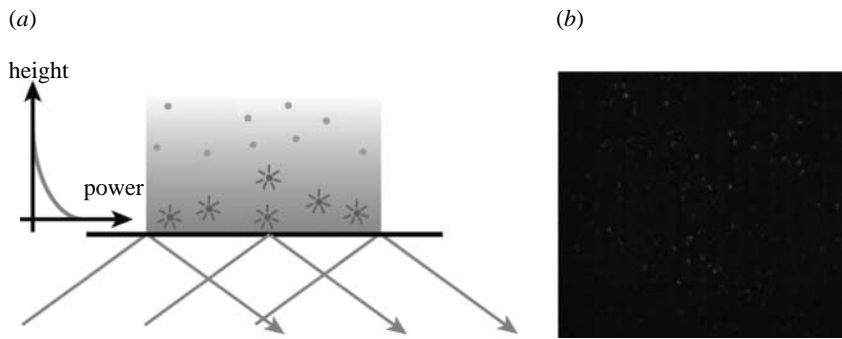
Figure 7. (a) Schematic of TIRF illumination. When the incidence angle is larger than the critical angle \theta_c , light is totally reflected and only the tracers closer than a fraction of the wavelength are illuminated. (b) Typical image of the tracers within the microchannel under TIRF illumination.
