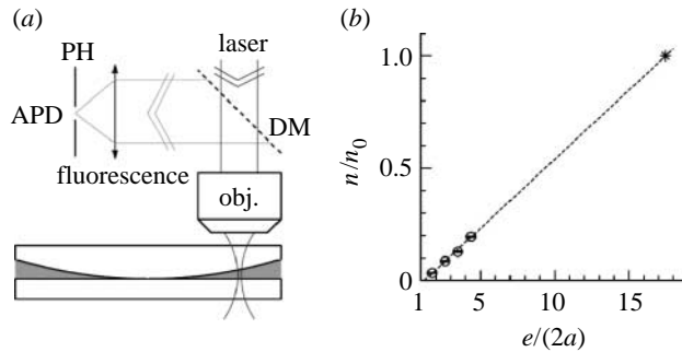
Figure 3. (a) Schematic of the experimental cell with FCS detection. Fluorescent colloids suspended in water are confined between a plane and a spherical lens. DM, dichroic mirror; obj., microscope objective; PH, pinhole; APD, avalanche photodiode. (b) Evolution of the bead number with the confinement. Symbol, polystyrene beads ( 2a=210 nm); dashed line, linear regression. Graph is taken from Joly et al. (2006).
