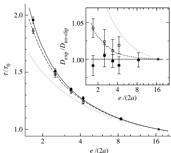
Figure 4. Evolution of the normalized diffusion time of silica beads ( 2a=218 nm) with confinement between a hydrophilic silica lens and a planar surface with varying surface property: filled circles, smooth hydrophilic surface (less than 1 nm peak-to-peak roughness); open squares, smooth hydrophobic wall (OTS-coated silica). Theoretical predictions are obtained using COMSOL, assuming no-slip on the lens, and different boundary conditions on the plane: solid lines, no-slip; dashed lines, partial slip with b=18 nm. As a guide, the dotted line shows the theoretical prediction for b=100 nm slip length, illustrating the method sensitivity. Graph is taken from Joly et al. (2006).
