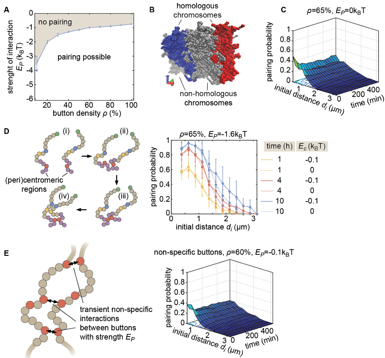
Figure 2 - Supplementary Figure 2. Properties of the button model. (A) Phase diagram representing parameter ranges resulting in simulations compatible (white area) and incompatible (grey area) with pairing, starting from favorable initial homologous chromosome configurations (aligned chromosomes with d_i < 1 \mu\text{m} , as in Fig. 2C). (B) Representative simulation snapshot for \rho=65\% and E_P=-1.6 k B T. When homologous chromosomes (red and blue monomers) are initially distant, steric hindrance by other chromosomes (grey monomers) may prevent pairing. (C) Behavior in the absence of specific interaction ( E_P=0 ) in the homologous button model. Predicted average pairing probability between euchromatic homologous loci (considered as paired if distance \leq 1 \mu\text{m} ) as a function of time and the initial distance d_i between homologous chromosomes. (D) Impact of HP1-mediated interaction between (peri)centromeric regions. (Left) Pairing between chromosomes that are initially distant (i) is facilitated and accelerated by the non-specific interactions between centromeric regions that lead to the clustering (ii) of HP1 regions. This clustering facilitates the pairing of homologous buttons located in centromeric regions (iii) and the subsequent pairing via the zipping process of nearby euchromatic regions (iv). (Right) Predicted average
