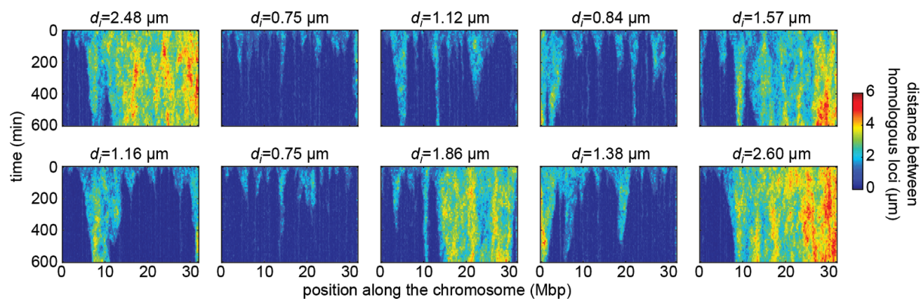
Figure 2 - Supplementary Figure 1. Simulated time evolution of distance between homologous loci. Examples of kymographs of the time-evolution of the distances between homologous regions predicted by the model in several simulated stochastic trajectories with different initial distances d_i for a button density of \varphi=65\% and an interaction strength of E_p=-1.6k_B T .
