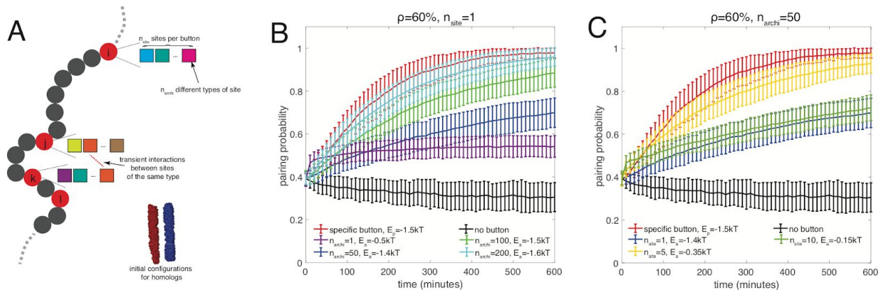
Discussion - Supplementary Figure 1. The combinatorial button model. (A) To investigate the possible nature of buttons, we developed a more general model where buttons are made of n_{site} binding sites for specific architectural proteins. Every site is occupied by one type of architectural proteins randomly chosen among n_{archi} different types. Two buttons may interact if they have common binding sites for some architectural proteins. The energy of a configuration is then given by
