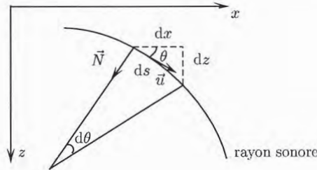
FIGURE 10 – Rayon sonore
