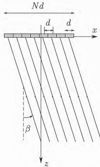
FIGURE 3 — Antenne multifaisceaux
