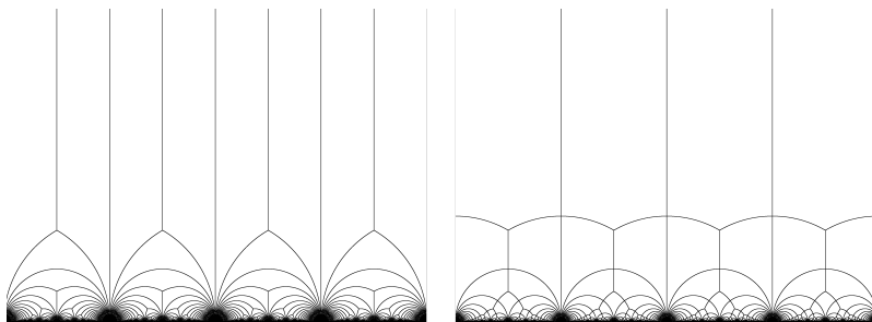
Figure VI.1: Two more tilings for \text{PSL}(2, \mathbb{Z}) (variants)
