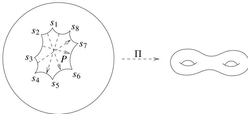
Figure VI.8: The surface of genus 2
