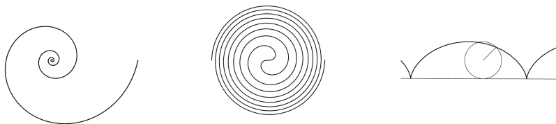
Figure 1: Some transcendental curves
