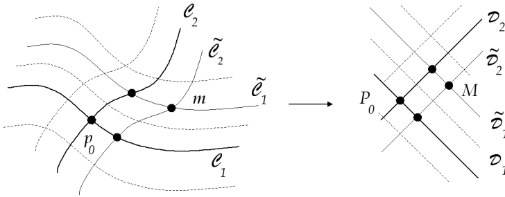
Figure I.6: The Lorentzian version of Gauss's theorem
