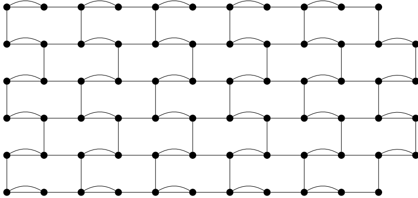
Figure 1: The graph \widehat{W}_5 .
