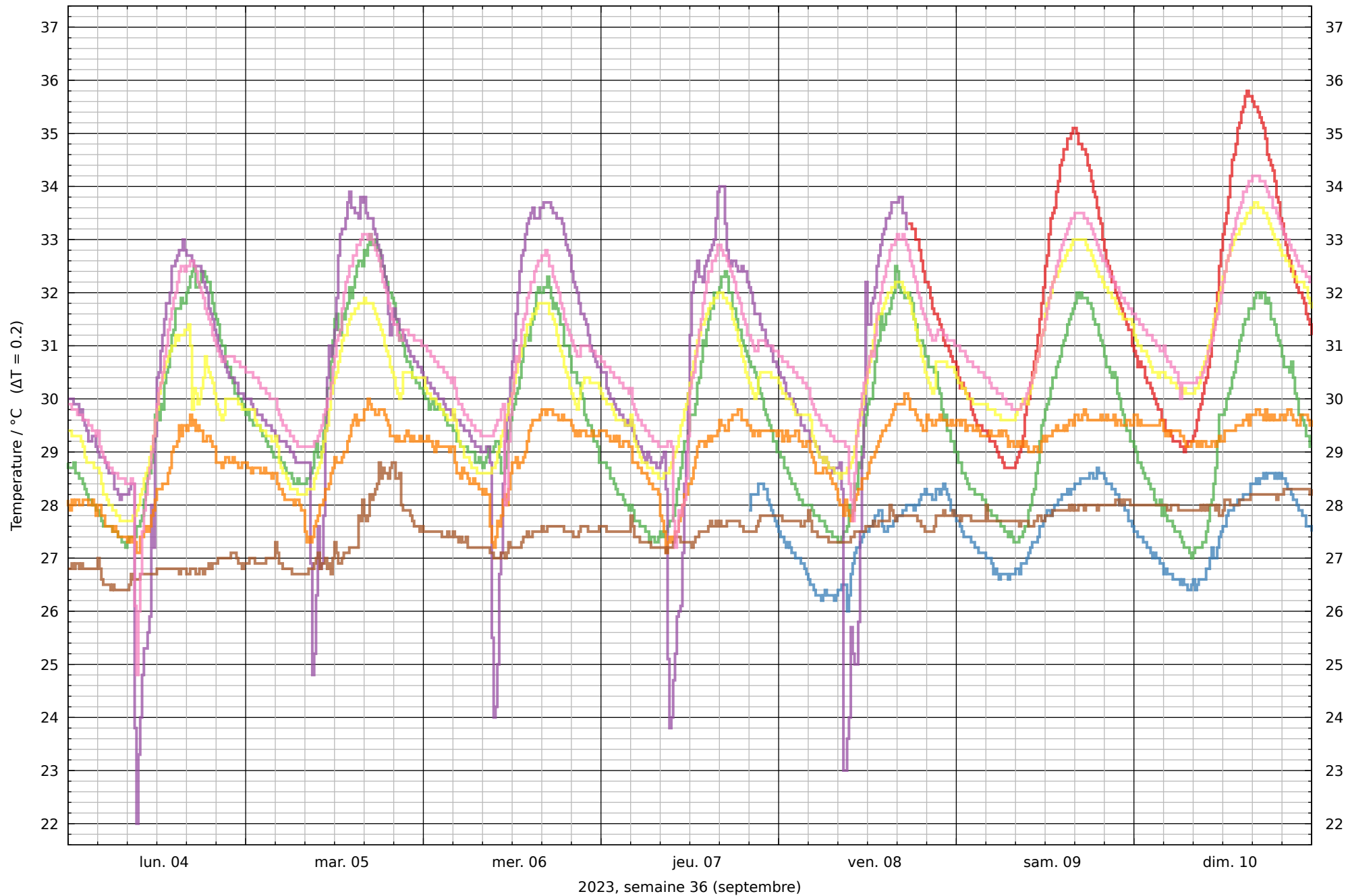
Temperature readings in LIP's offices ( \Delta t = 4h , black line = midnight)
