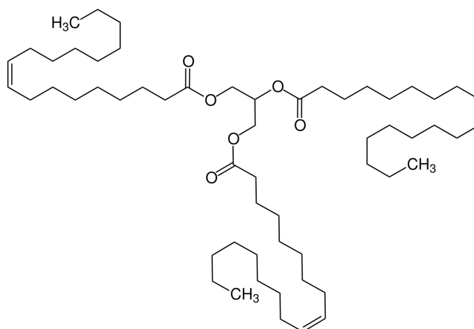
FIGURE 6 – Trioléine
