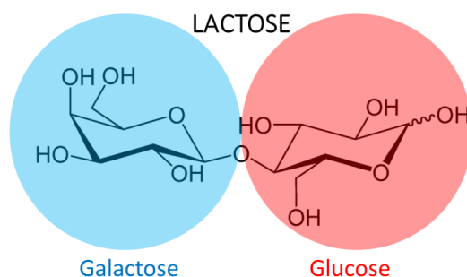
FIGURE 4 – lactose
