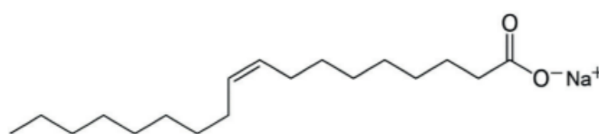
FIGURE 7 – Ion oléine
