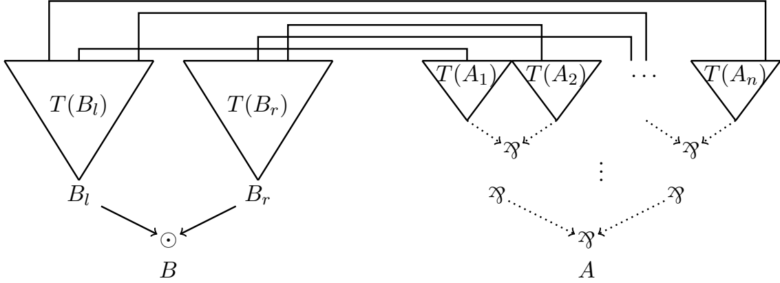
Figure 15: Proof-net of Lemma 8.33 with all terminal \&mathcal{A} -vertices removed
