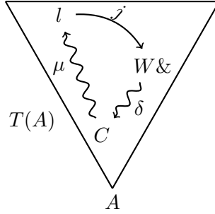
Figure 7: Illustration of the proof of Lemma 8.13
