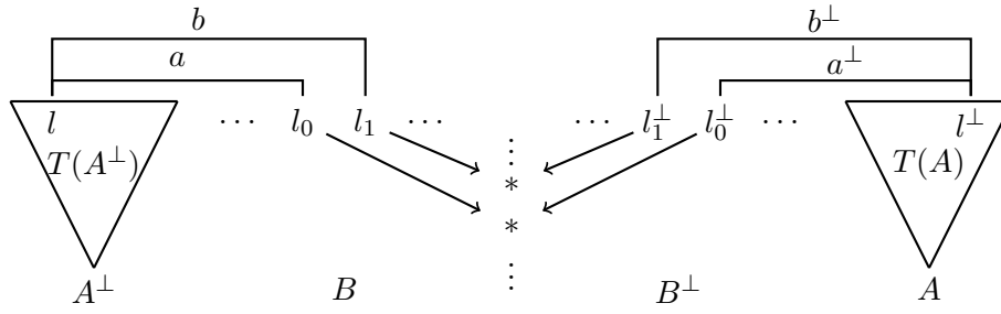
Figure 12: Almost reduced composition \psi of \theta and \theta' by cut over B in the proof of Theorem 8.19
