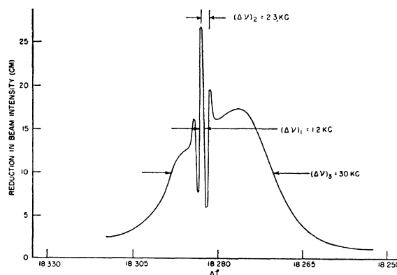
FIG. 3. Experimentally observed reduction in beam intensity as a function of frequency. Line 2,0 \rightarrow 1,0 K^{39} ; H=1.5 gauss; I_{RF} \approx 8 ma; F = F^0 - \Delta F ; F^0 = 479.27 mc; total beam intensity = 216 cm.
