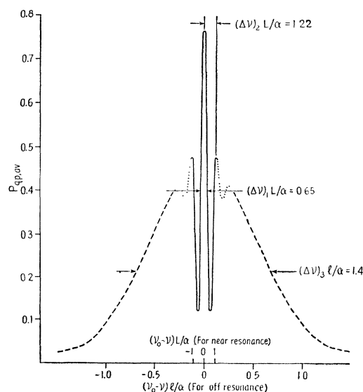
FIG. 2. Transition probability as a function of frequency. ——— Calculated near resonance. ----- Calculated off resonance. .... Interpolated.
