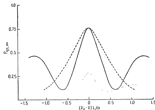
FIG. 1. Transition probability as a function of frequency near resonance. L = distance between oscillating field regions. \alpha = most probable molecule velocity. \nu = oscillator frequency. — New method with maximum transition probability. ···· Same with one-third the strength of oscillating field. ---- Previous method with maximum transition probability.
