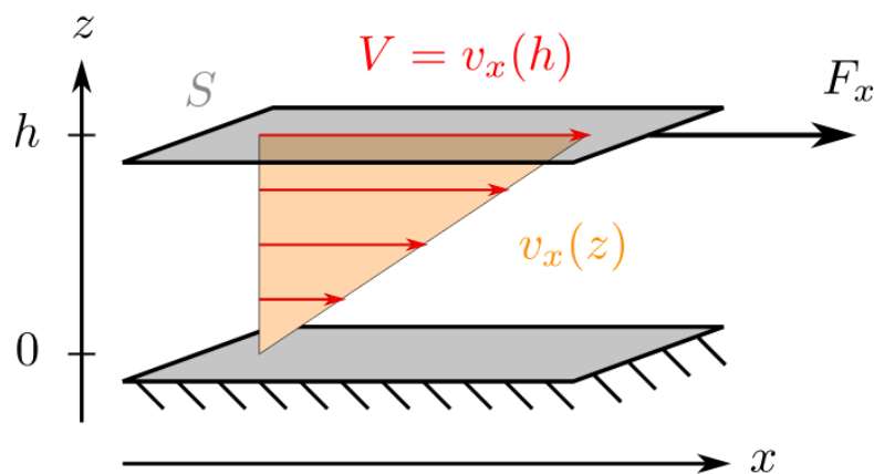
FIGURE 1 – Ecoulement Couette plan
