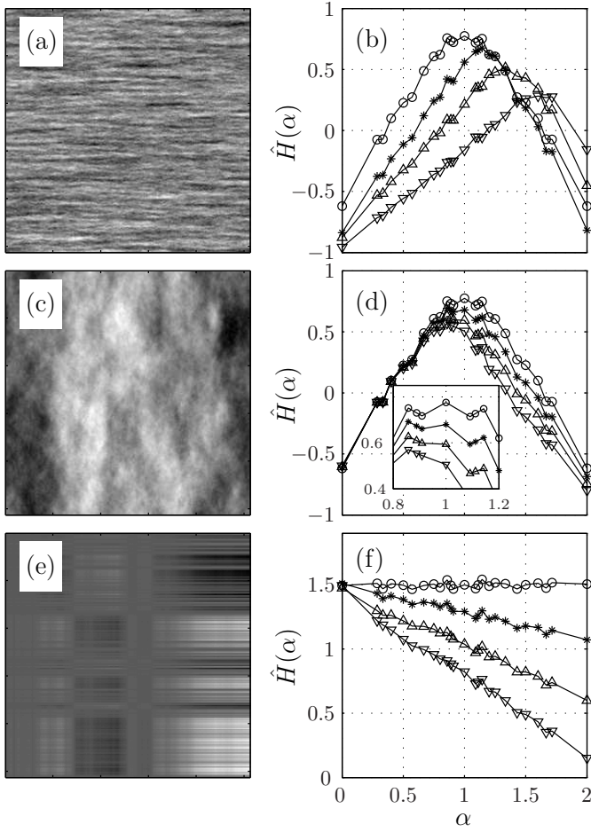
Fig. 8. Other (an)isotropic selfsimilar Gaussian fields. (a, c, e) sample fields with (H_1, H_2) = (0.2, 0.8) for OSGRF (a), EFBF (c), FBS (e). (b, d, f) : \hat{H}(\alpha) obtained for averages over 100 realizations, with H_2 = 0.8 and H_1 = 0.8 ( \circ ), 0.6 ( \star ), 0.4 ( \Delta ) and 0.2 ( \nabla ). \hat{H}(\alpha) clearly shows a maximum for \alpha \neq 1 when fields are anisotropic.
