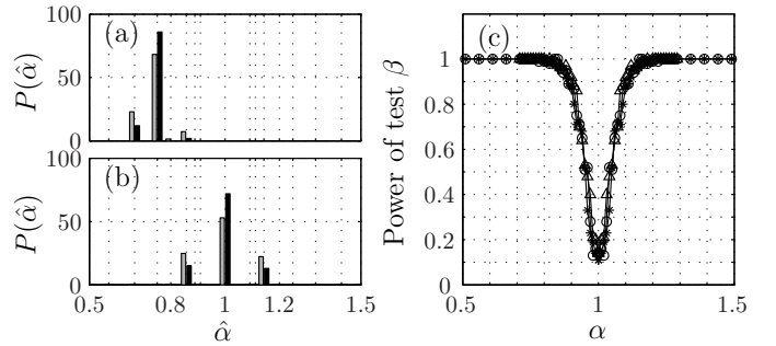
Fig. 7. Anisotropy test. a) Histogram of \hat{\alpha}_{MC} (light gray) and of \hat{\alpha}_{BS} (black) for OSGRF X_{0, \alpha_0, H_0} (image size (2^{10}, 2^{10}) ), with \alpha_0 = 0.75 (a) and \alpha_0 = 1 (b). Right plot (c) shows the rejection level of the test (with a significance level of 90%) obtained for R = 100 bootstraps, averaged on 100 realizations of X_{0, \alpha_0, H_0} , with H_0 = 0.3 (o), 0.5 ( \Delta ) and 0.7 ( \nabla ).
