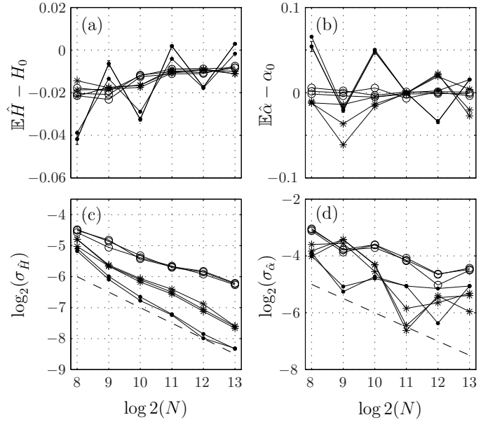
Fig. 4. Estimation performance. As functions of the sample size N (image size N \times N ), biases (top row) and standard deviation for \hat{H}_{q=2} (a, c) and \hat{\alpha}_{q=2} (b, d), obtained as average of estimation performed on 500 realizations of OSGRF X_{0, \alpha_0, H_0} with parameters \alpha_0 = 1, H_0 = 0.7, 0.5 and 0.3 ( \circ ), \alpha_0 = 0.8, H_0 = 0.7, 0.5, 0.3 ( * ) and \alpha_0 = 0.6, H_0 = 0.5, 0.3 ( \cdot ). In (c) and (d), dashed lines illustrates the expected 1/\sqrt{N} decrease of the standard deviations.
