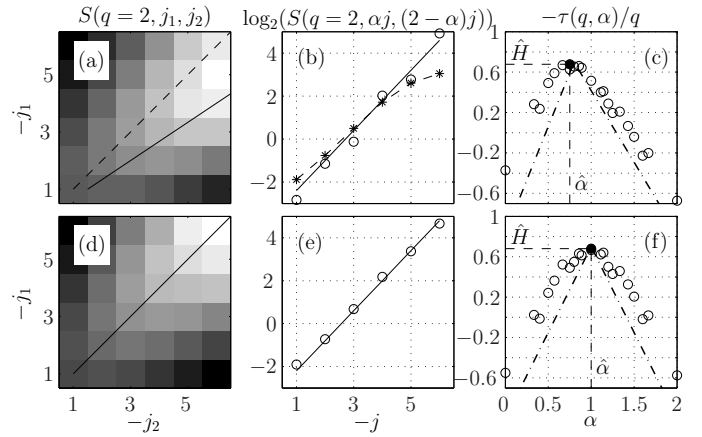
Fig. 3. Illustrations of the estimation procedures. For anisotropic, \alpha_0 = 0.7 (a,b, c), and isotropic, \alpha_0 = 1 (d,e,f), OSGRF X_{\theta_0, \alpha_0, H_0} , with \theta_0 = 0 , H_0 = 0.7 . (a, d): Structure functions S(q, j_1, j_2) . The solid line indicates the direction \hat{\alpha} while the dashed lines correspond to \alpha = 1 and hence the sole direction actually reachable with the coefficients of 2D-DWT. (b, e): Estimation of H(\alpha) , based on \tau(q=2, \alpha = \hat{\alpha}) obtained from a linear regression of \log_2 S(q, \alpha j, (2-\alpha)j) versus j (o). Solid lines correspond to the theoretical -\tau(q=2, \alpha_0) . Stars (in (b)) correspond to the (biased) estimation of H from -\tau(q=2, \alpha=1) , i.e. by using only the 2D-DWT coefficients. (c, f): Plots of \hat{H}_2(\alpha) = -\tau(2, \alpha)/2 versus \alpha . The black dot shows the location of the maximum of H_2(\alpha) = -\tau(2, \alpha)/2 thus yielding the estimated \hat{\alpha} and \hat{H} . In (f), as expected for an isotropic image, \hat{\alpha} = 1 . The mixed line corresponds to the theoretical values of -\tau(2, \alpha)/2 (cf. Eq. 11).
