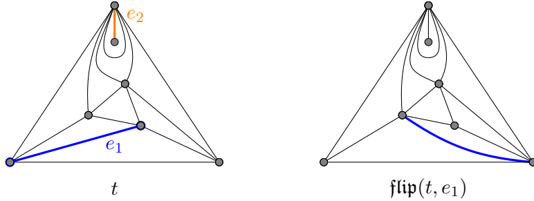
Figure 1: An example of flip of an edge. The orange edge e_2 is not flippable.
