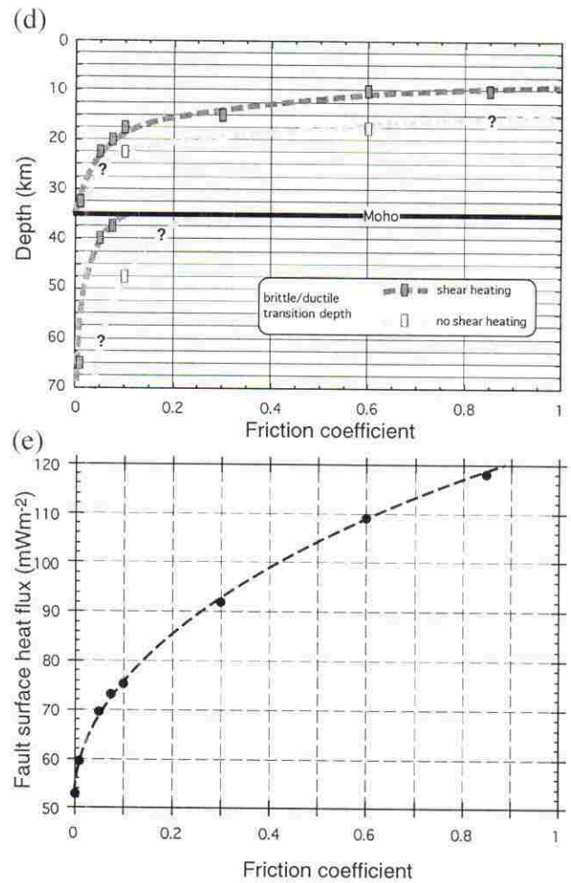
Figure 9. (Continued.)
