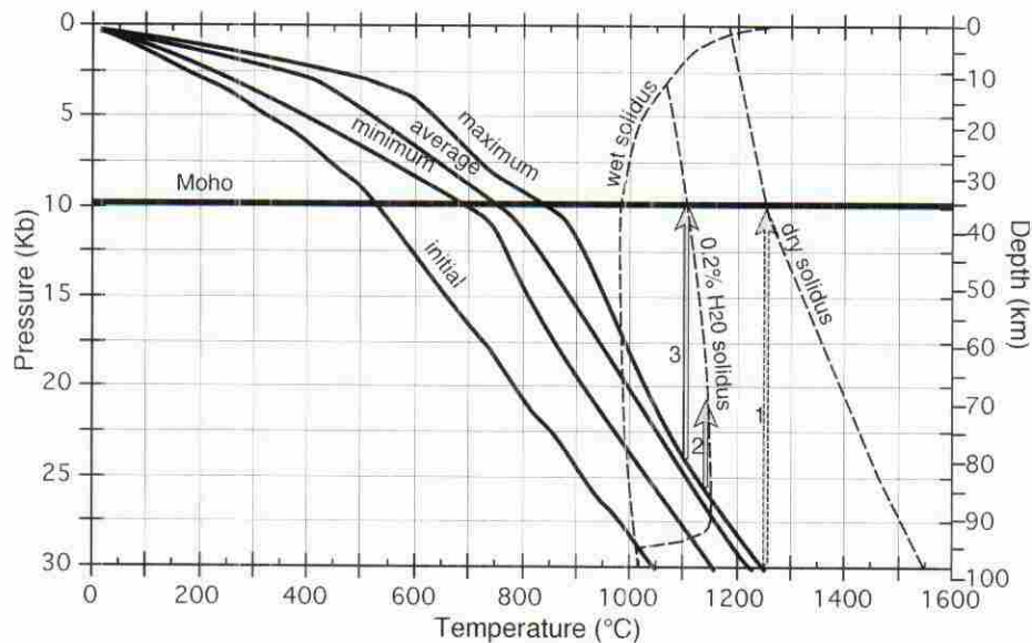
Figure 13. Shear-zone lithospheric geotherms calculated for a 4 \text{ cm yr}^{-1} shear rate compared with peridotite melting curves. Steady-state model geotherms. Same as in Fig. 12. Simplified upper mantle melting curves. Wet solidus: \text{H}_2\text{O} -saturated peridotite (Kushiro et al. 1968); dry solidus: dry peridotite solidus (Wyllie 1971); solidus for pyrolite with \approx 0.2 per cent \text{H}_2\text{O} (Green 1973). Arrows 2 and 3 correspond to possible decompression paths leading from a shear-heating geotherm to mantle partial fusion in the case of a slightly hydrous upper mantle. Note that such decompression melting is impossible if starting from the initial geotherm.
