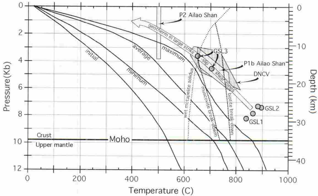
Figure 12. Shear-zone crustal geotherms calculated for a 4 \text{ cm yr}^{-1} shear rate compared with thermobarometric data of ASRR and GSL shear zones and crustal melting curves. Steady-state model geotherms. Initial: reference model before shearing; Average: V = 4 \text{ cm yr}^{-1} , otherwise reference parameters; maximum: maximum shear heating for V = 4 \text{ cm yr}^{-1} ( F = 0.6 , hard crust, hard mantle); Minimum: minimum shear heating for V = 4 \text{ cm yr}^{-1} ( F = 0.1 , soft crust, soft mantle). Simplified crustal melting curves. Wet solidus: \text{H}_2\text{O} -saturated metapelite solidus (Thompson 1982); Muscovite breakdown: muscovite dehydration melting ( \text{Mus} + \text{Alb} + \text{Q} \rightarrow \text{Ksp} + \text{Als} + \text{L} ) (Petö 1976); Biotite break-down: biotite dehydration melting ( \text{Bio} + \text{Als} + \text{Pl} + \text{Q} \rightarrow \text{Gar} + \text{Ksp} + \text{L} ) (Le Breton & Thompson 1988). P-T estimates. ASRR shear zone: Peak (P1b and DNCV) and retrograde (P2) paragenesis (Leloup & Kienast 1993; Leloup, unpublished data); Great slave lake shear zone (GSL): GSL1, 2 and 3 correspond to P-T estimates in the granulite, upper amphibolite and amphibolite belts of the shear zone, respectively (Hanmer 1988).
